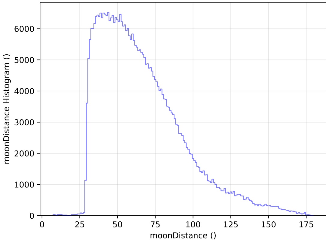
roll_pause_mjdp270_v3.4_10yrs WFD y band: moonDistance Histogram
