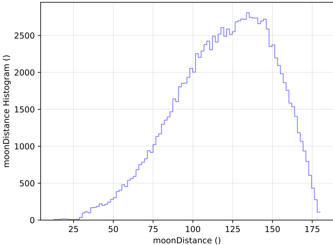
roll_pause_mjdp270_v3.4_10yrs WFD u band: moonDistance Histogram
