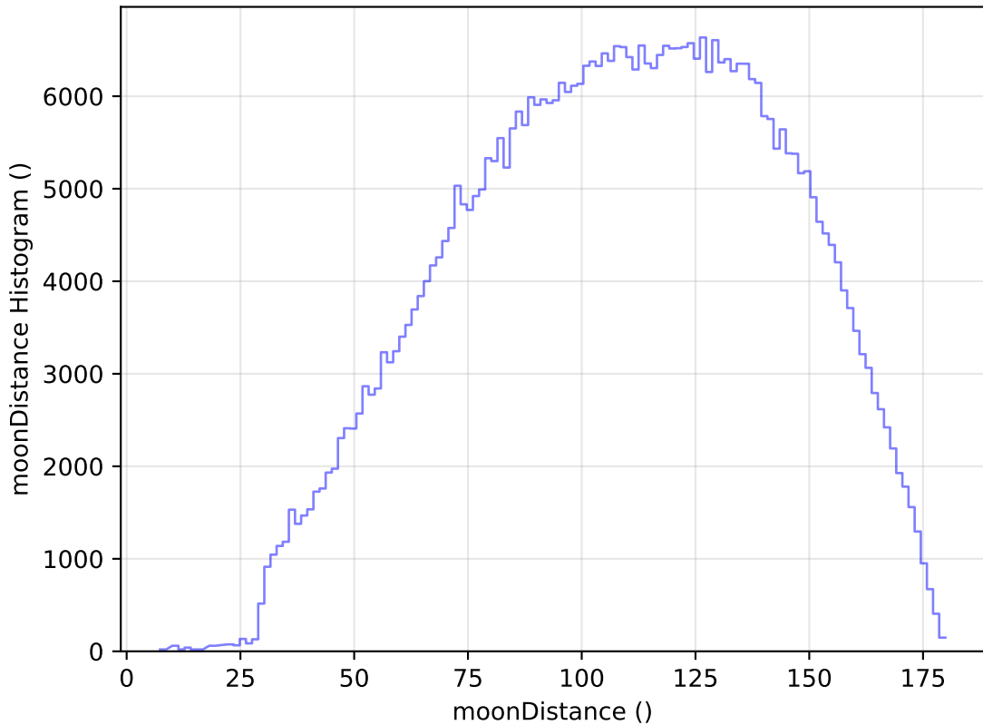
roll_pause_mjdp270_v3.4_10yrs WFD r band: moonDistance Histogram
