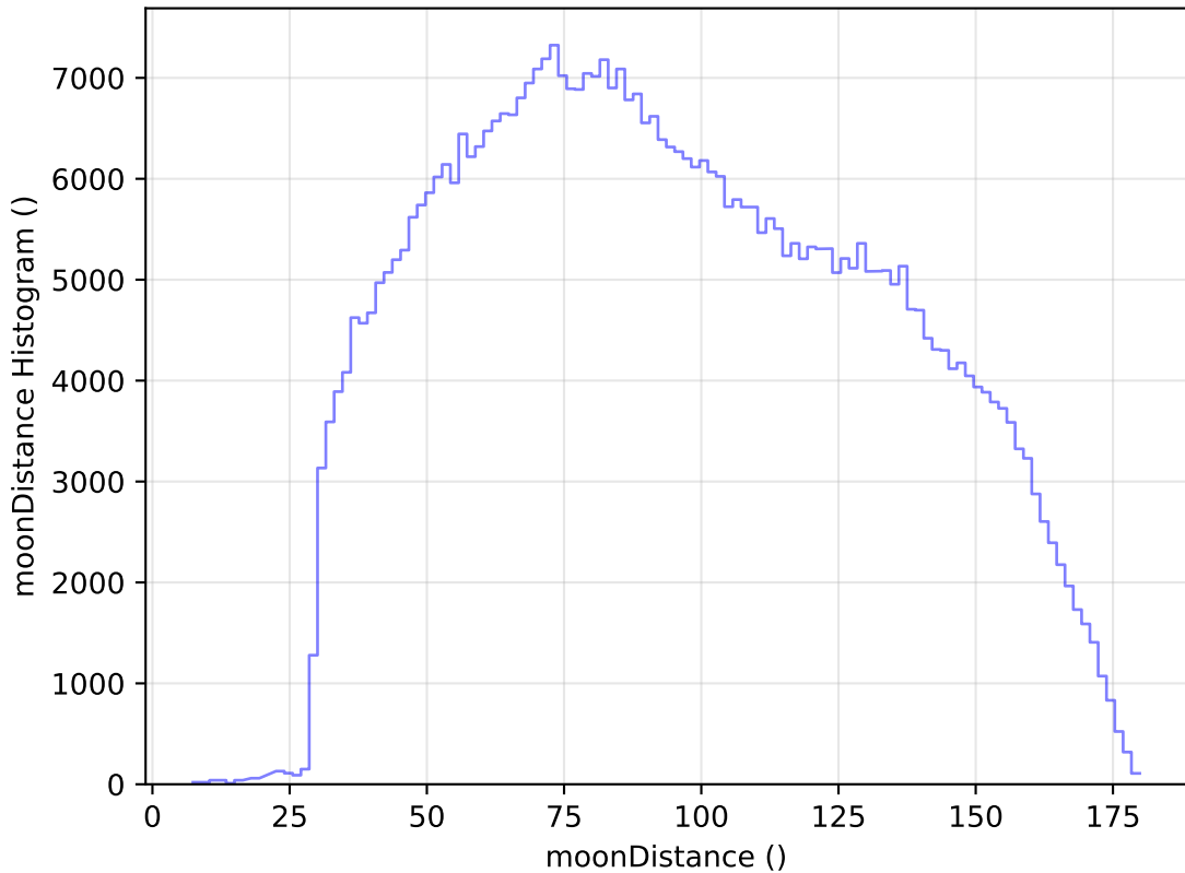
roll_pause_mjdp270_v3.4_10yrs WFD i band: moonDistance Histogram
