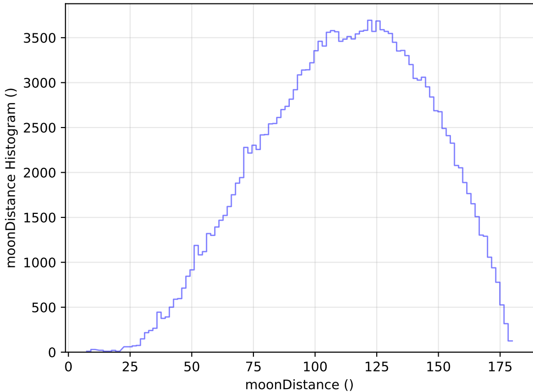
roll_pause_mjdp270_v3.4_10yrs WFD g band: moonDistance Histogram
