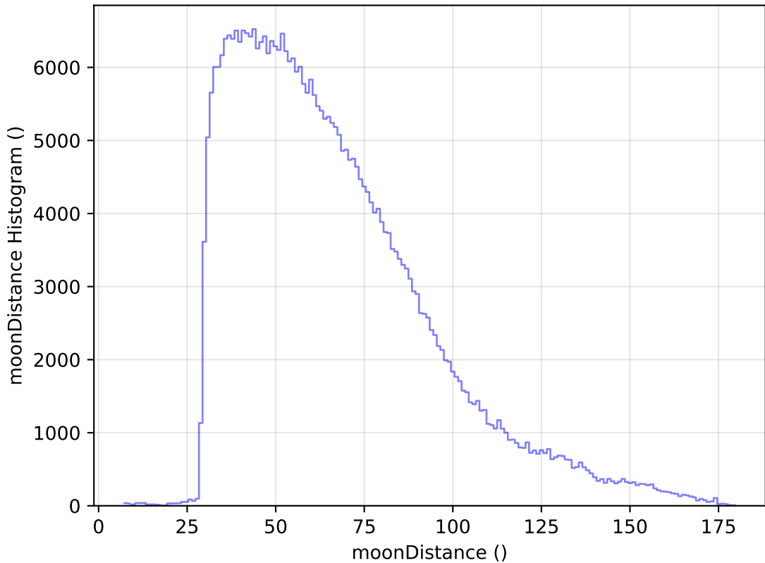
roll_pause_mjdp270_v3.4_10yrs All sky y band: moonDistance Histogram
