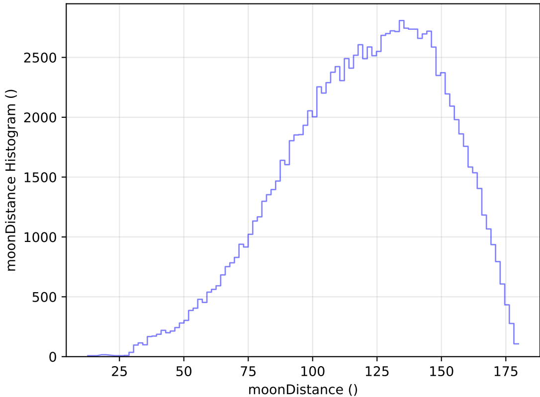
roll_pause_mjdp270_v3.4_10yrs All sky u band: moonDistance Histogram
