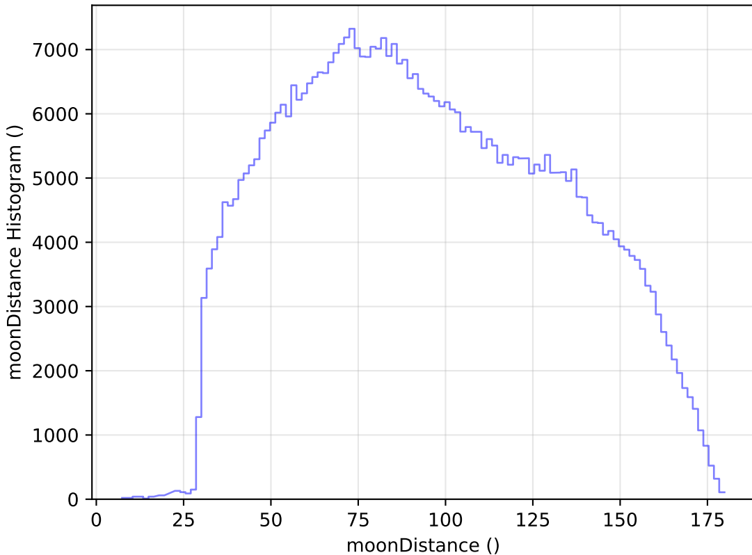
roll_pause_mjdp270_v3.4_10yrs All sky i band: moonDistance Histogram
