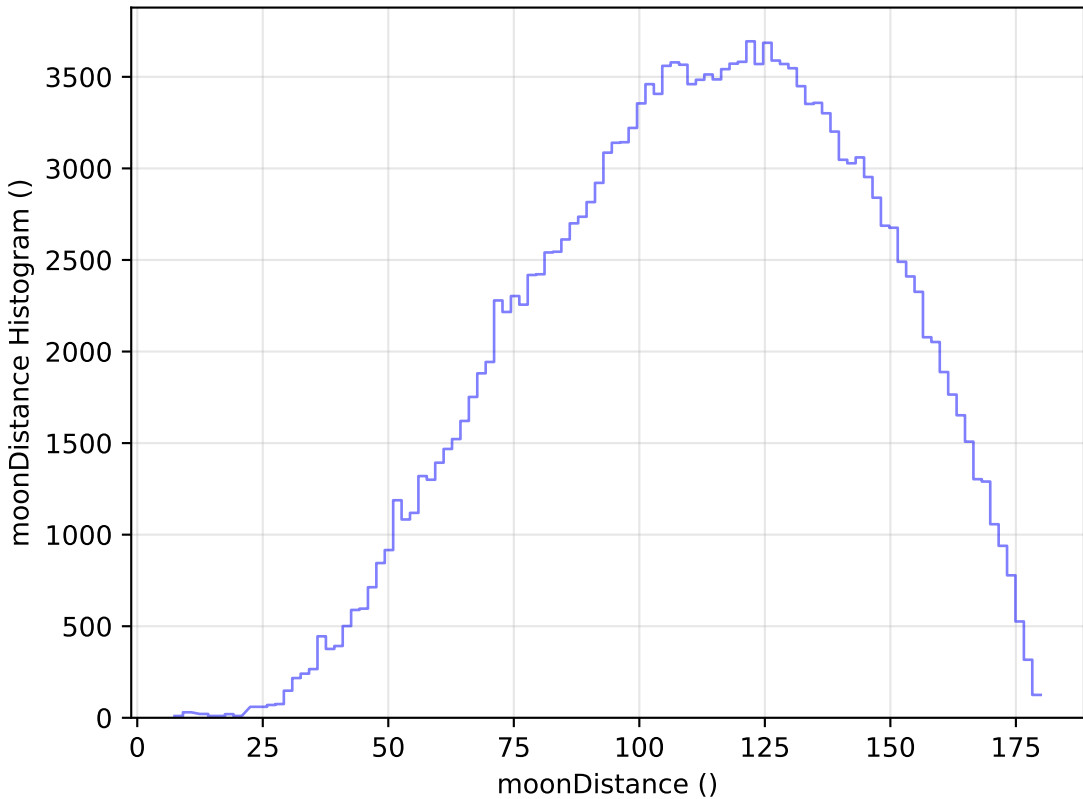
roll_pause_mjdp270_v3.4_10yrs All sky g band: moonDistance Histogram
