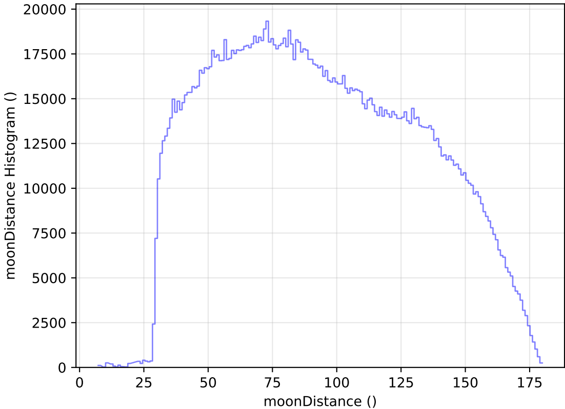
roll_pause_mjdp270_v3.4_10yrs All sky all bands: moonDistance Histogram
