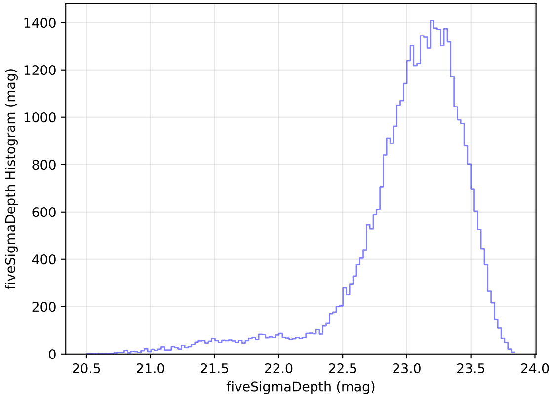
roll_pause_mjdp270_v3.4_10yrs Yr 1 z band: fiveSigmaDepth Histogram
