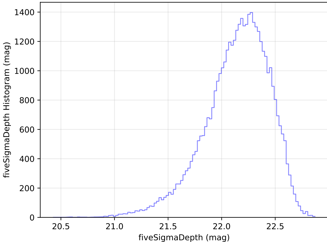
roll_pause_mjdp270_v3.4_10yrs Yr 1 y band: fiveSigmaDepth Histogram
