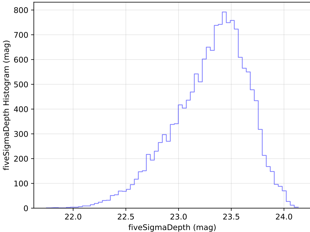
roll_pause_mjdp270_v3.4_10yrs Yr 1 u band: fiveSigmaDepth Histogram
