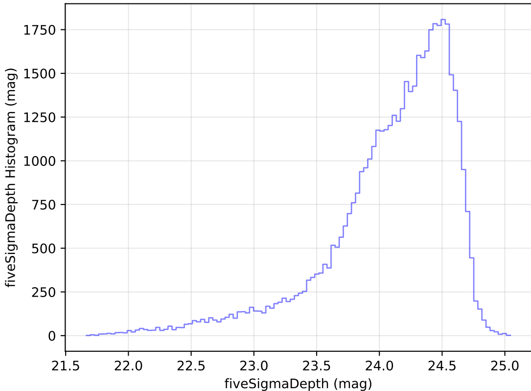
roll_pause_mjdp270_v3.4_10yrs Yr 1 r band: fiveSigmaDepth Histogram
