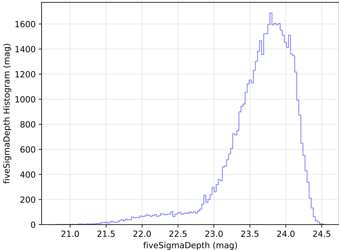
roll_pause_mjdp270_v3.4_10yrs Yr 1 i band: fiveSigmaDepth Histogram
