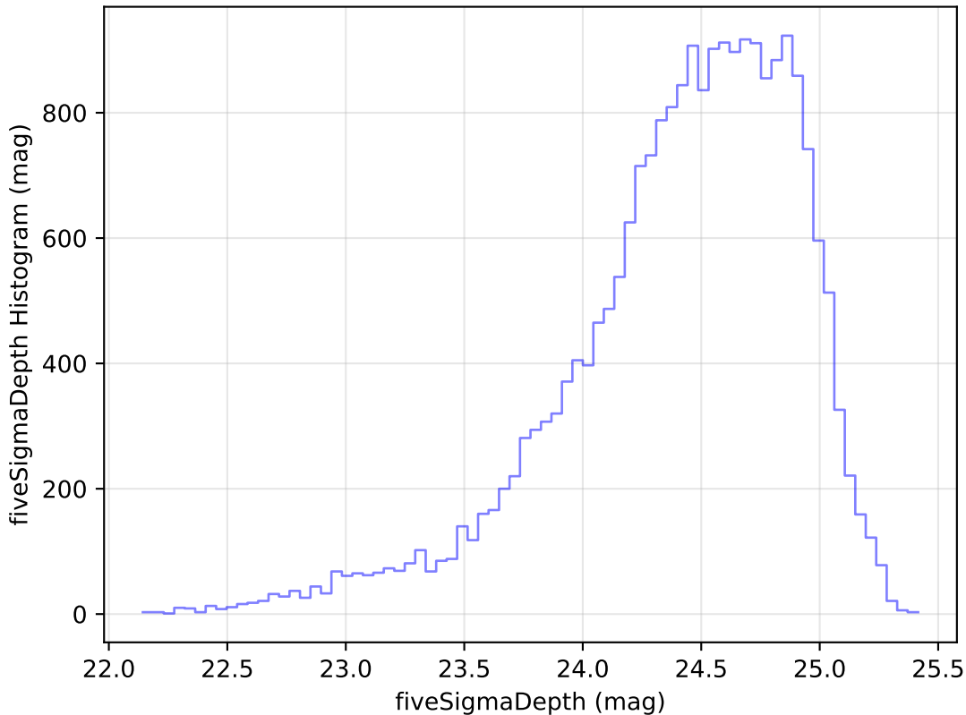
roll_pause_mjdp270_v3.4_10yrs Yr 1 g band: fiveSigmaDepth Histogram
