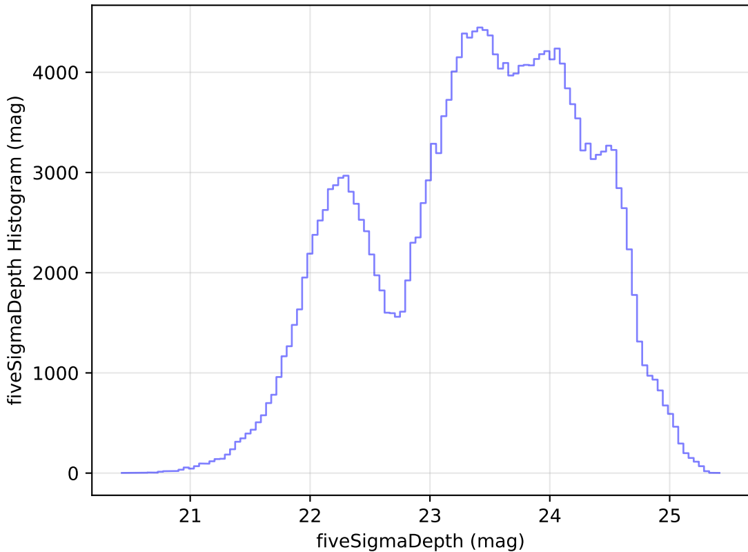
roll_pause_mjdp270_v3.4_10yrs Yr 1 all bands: fiveSigmaDepth Histogram
