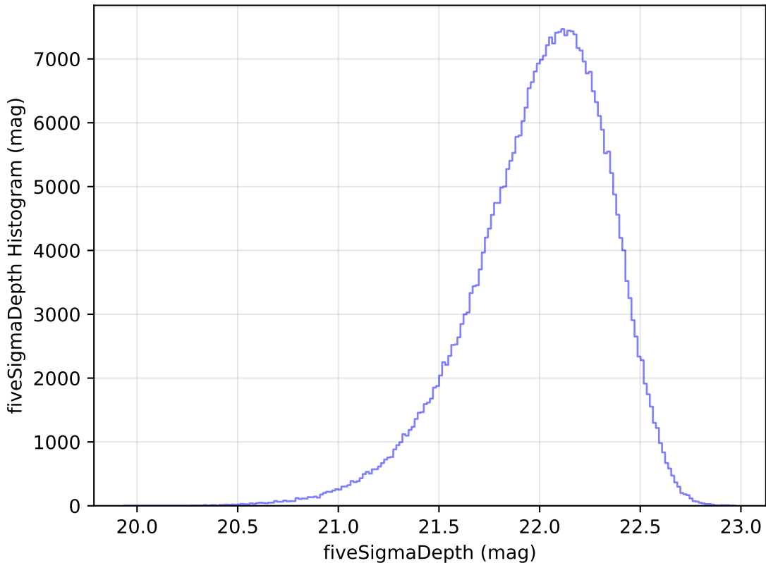
roll_pause_mjdp270_v3.4_10yrs WFD y band: fiveSigmaDepth Histogram
