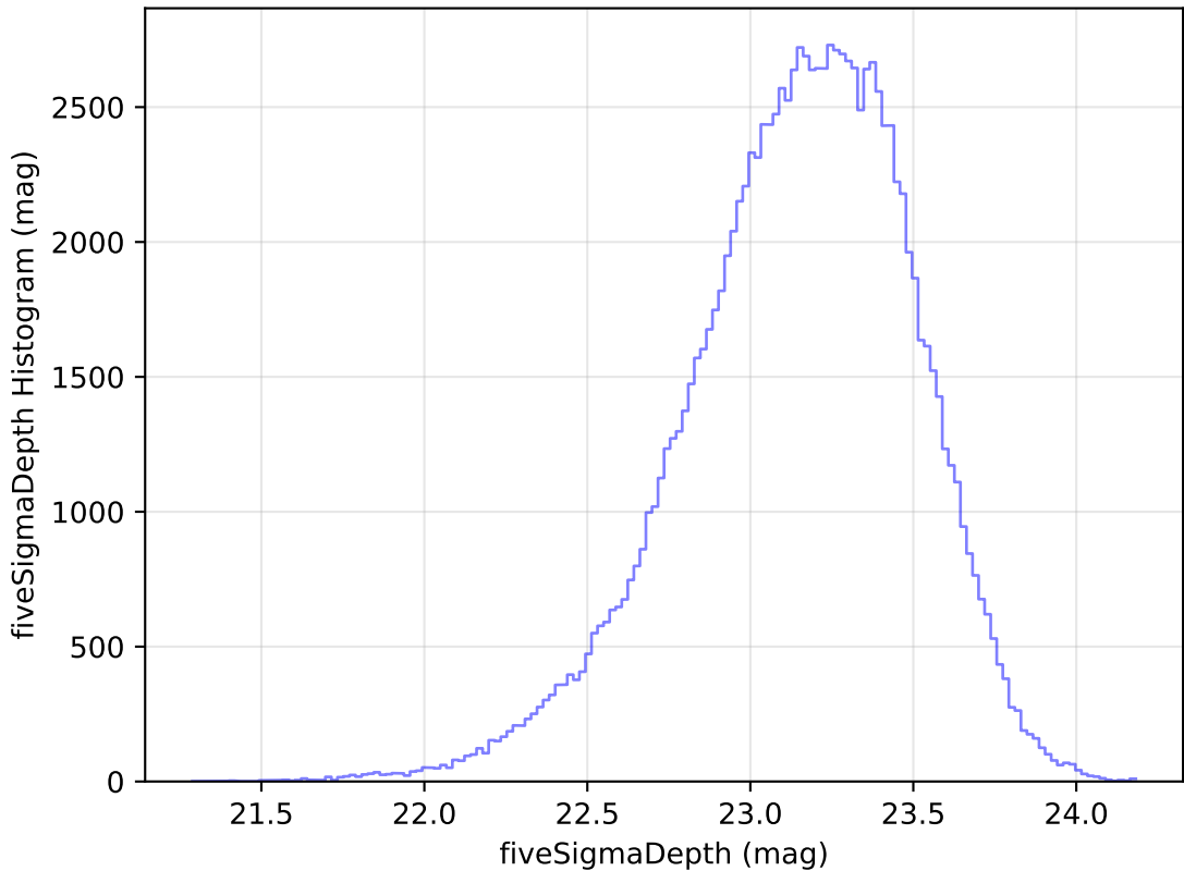
roll_pause_mjdp270_v3.4_10yrs WFD u band: fiveSigmaDepth Histogram
