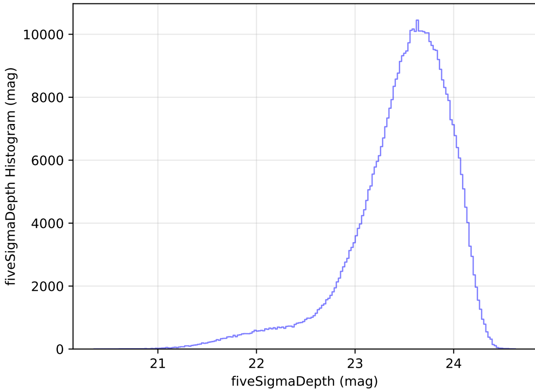
roll_pause_mjdp270_v3.4_10yrs WFD i band: fiveSigmaDepth Histogram
