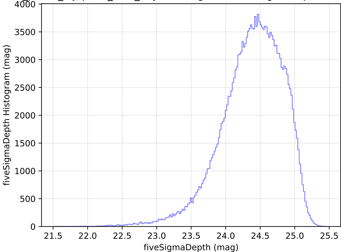
roll_pause_mjdp270_v3.4_10yrs WFD g band: fiveSigmaDepth Histogram
