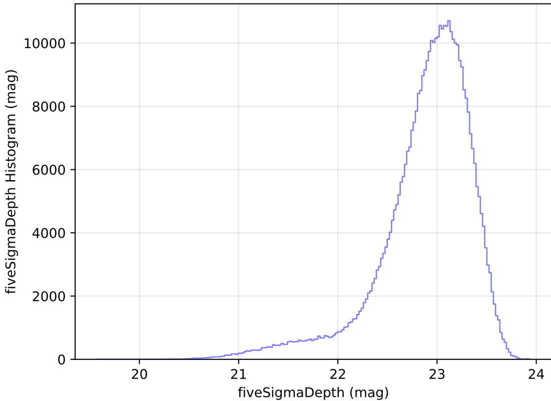
roll_pause_mjdp270_v3.4_10yrs All sky z band: fiveSigmaDepth Histogram
