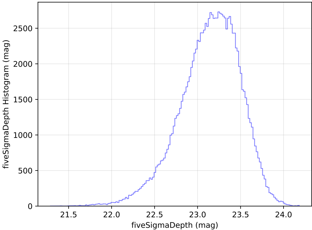
roll_pause_mjdp270_v3.4_10yrs All sky u band: fiveSigmaDepth Histogram
