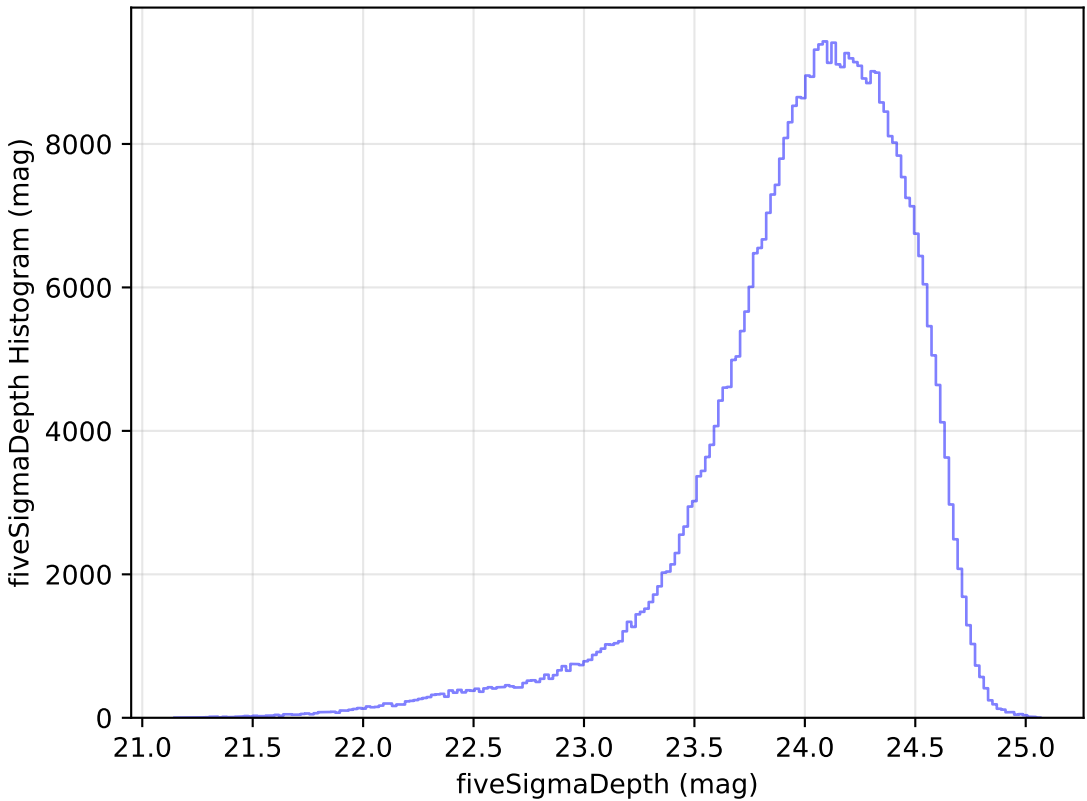
roll_pause_mjdp270_v3.4_10yrs All sky r band: fiveSigmaDepth Histogram
