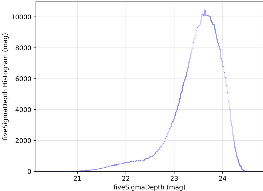
roll_pause_mjdp270_v3.4_10yrs All sky i band: fiveSigmaDepth Histogram
