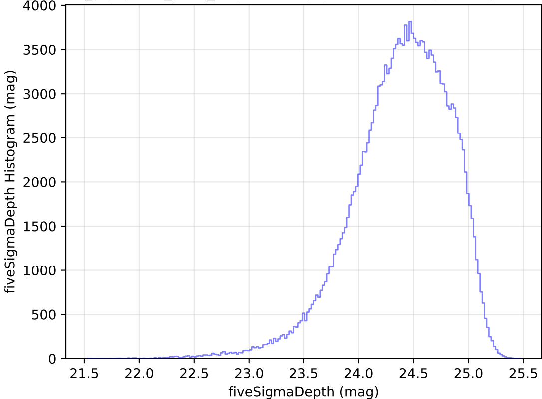
roll_pause_mjdp270_v3.4_10yrs All sky g band: fiveSigmaDepth Histogram
