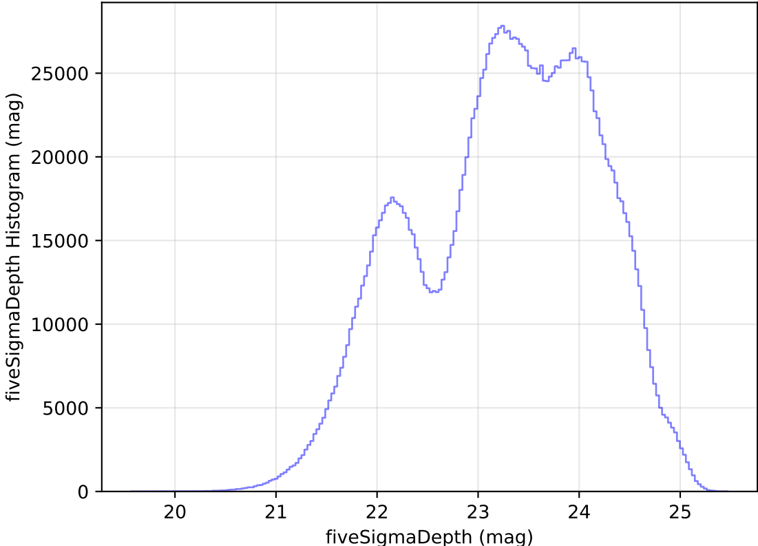
roll_pause_mjdp270_v3.4_10yrs All sky all bands: fiveSigmaDepth Histogram
