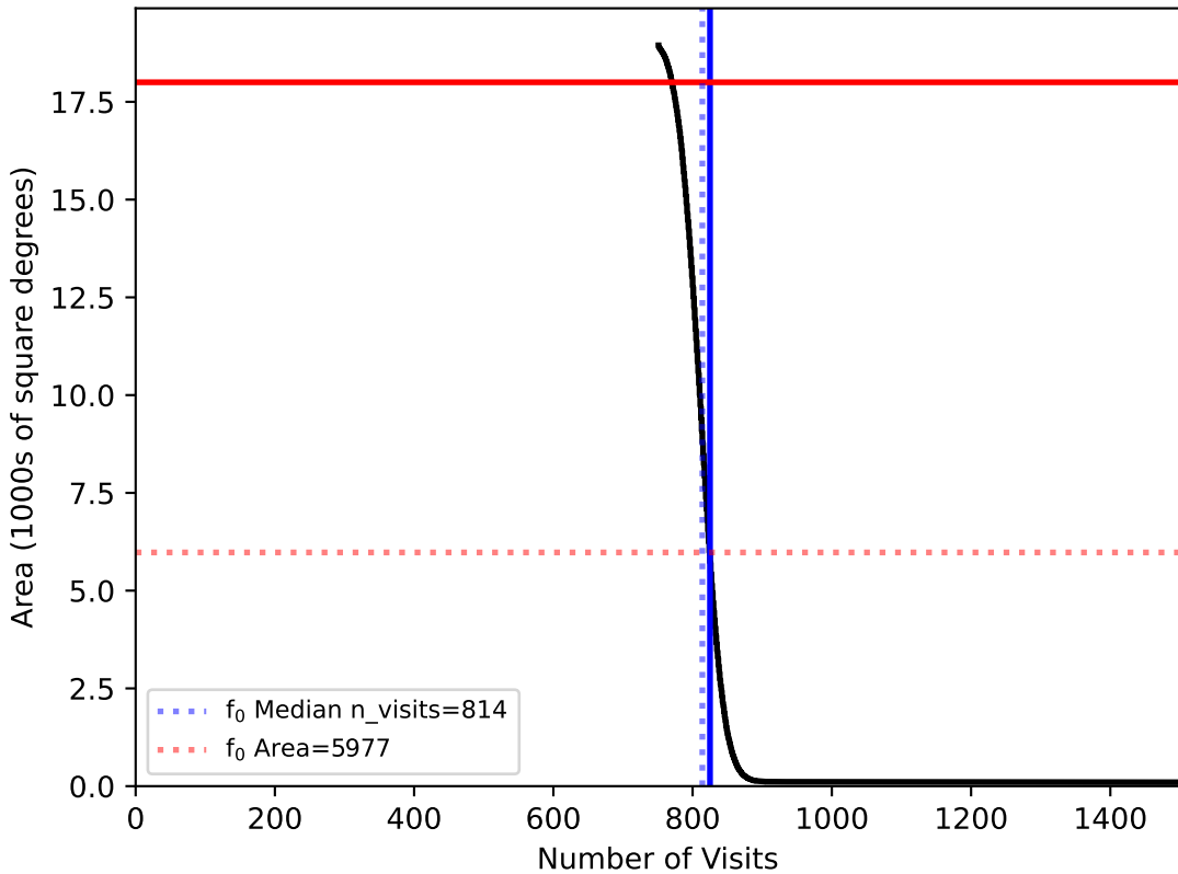
roll_pause_mjdp270_v3.4_10yrs WFD: f0
