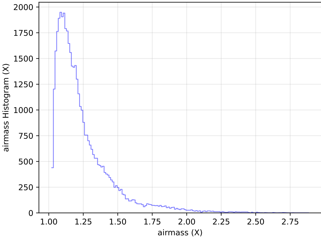
roll_pause_mjdp270_v3.4_10yrs Yr 1 y band: airmass Histogram
