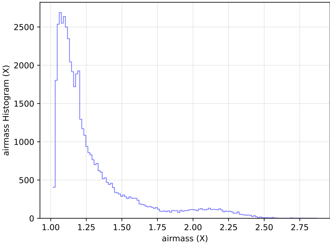
roll_pause_mjdp270_v3.4_10yrs Yr 1 r band: airmass Histogram
