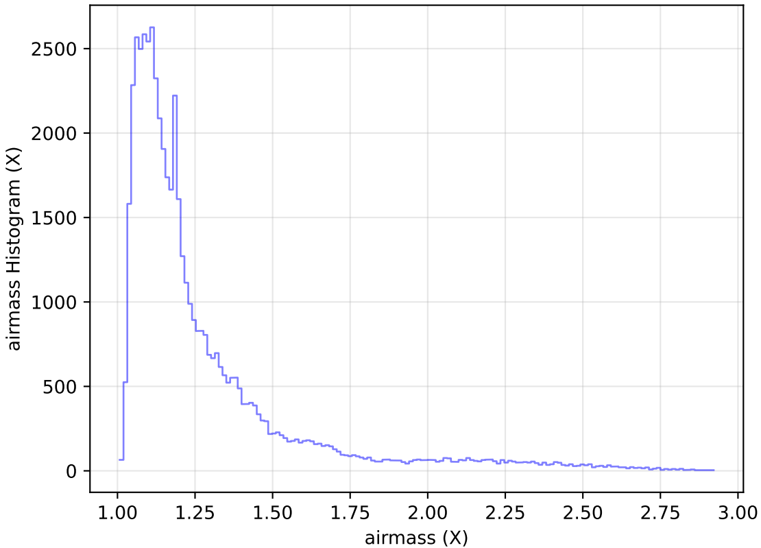
roll_pause_mjdp270_v3.4_10yrs Yr 1 i band: airmass Histogram
