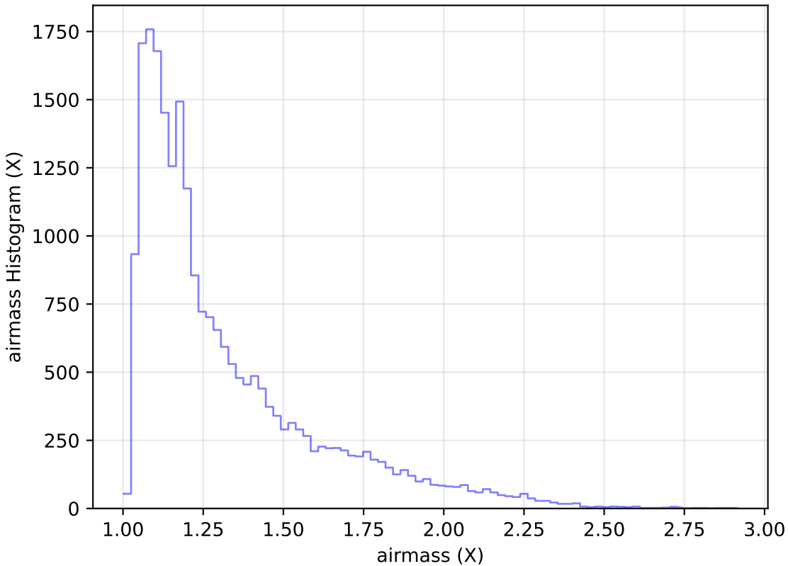
roll_pause_mjdp270_v3.4_10yrs Yr 1 g band: airmass Histogram
