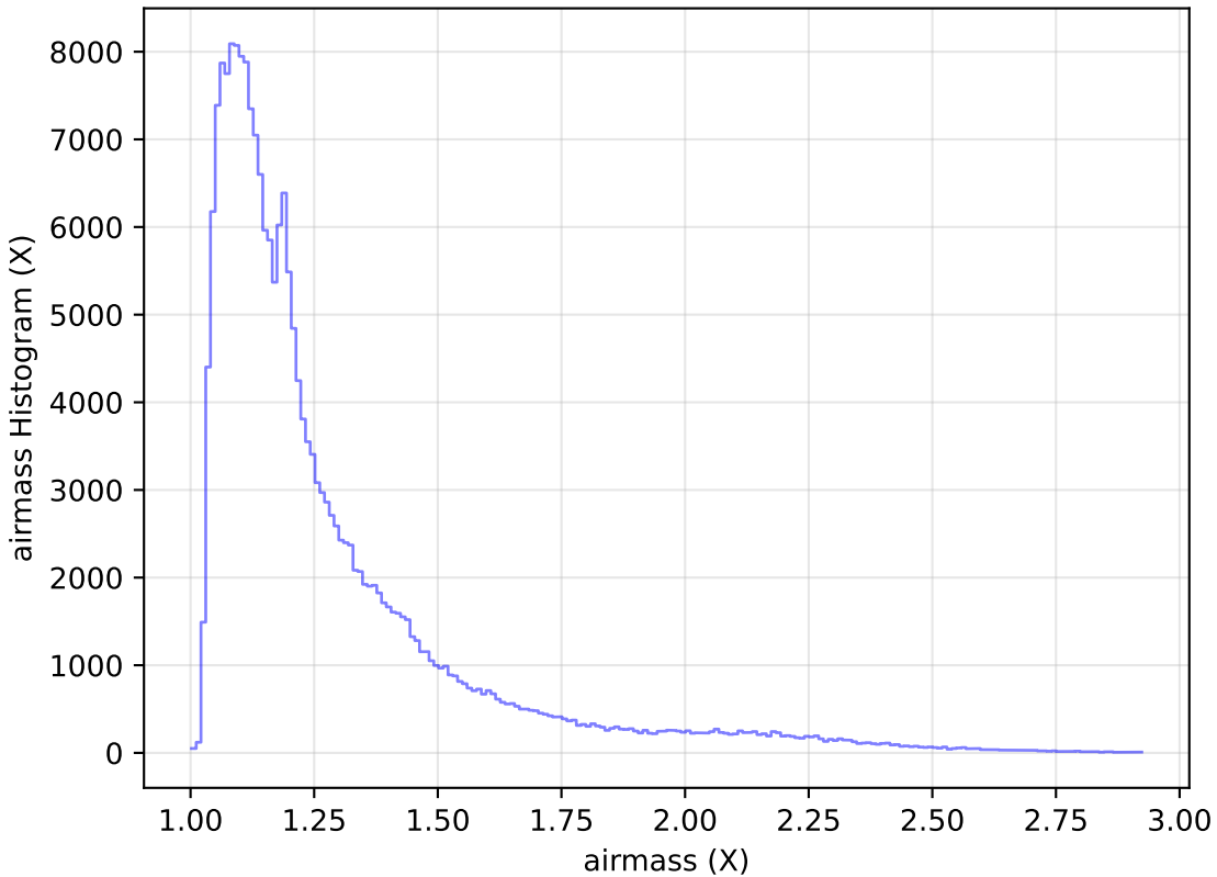
roll_pause_mjdp270_v3.4_10yrs Yr 1 all bands: airmass Histogram
