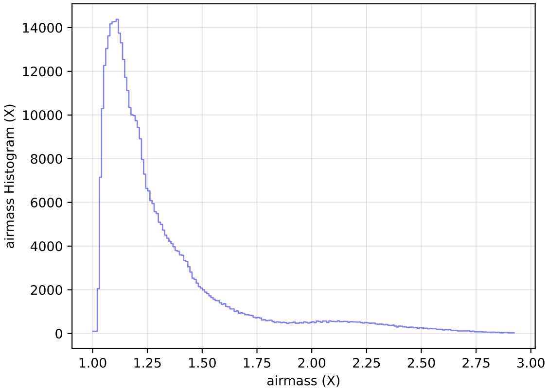
roll_pause_mjdp270_v3.4_10yrs WFD z band: airmass Histogram
