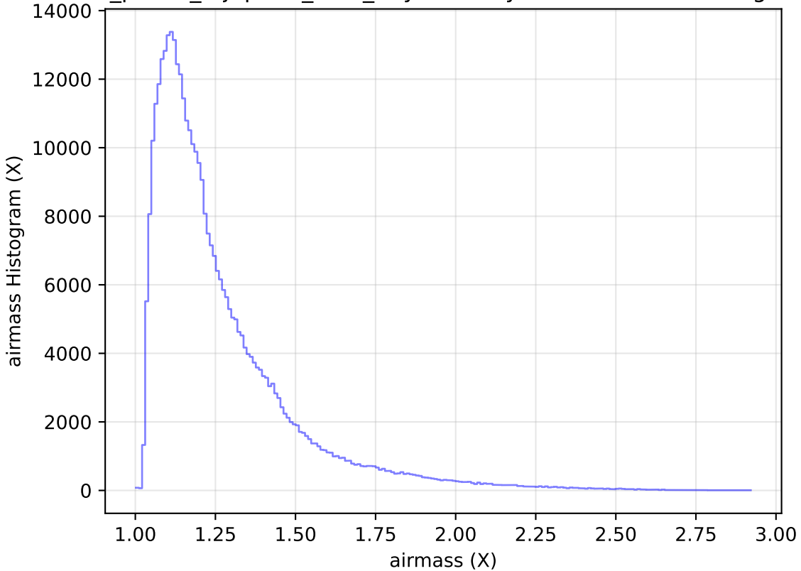
roll_pause_mjdp270_v3.4_10yrs WFD y band: airmass Histogram
