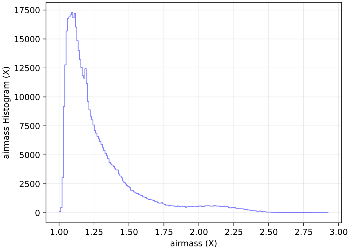
roll_pause_mjdp270_v3.4_10yrs WFD r band: airmass Histogram
