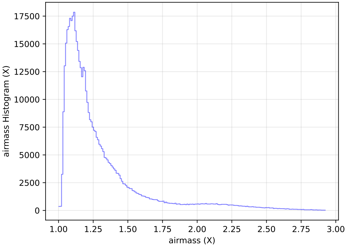
roll_pause_mjdp270_v3.4_10yrs WFD i band: airmass Histogram
