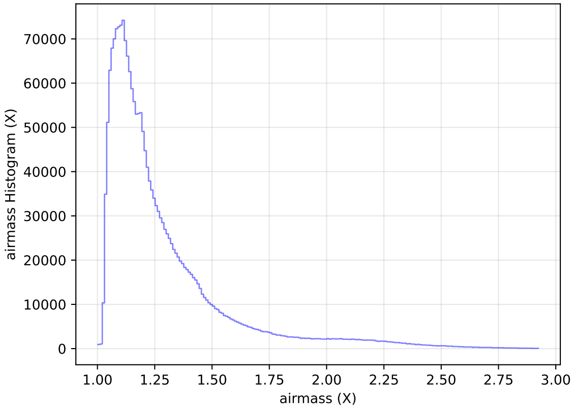
roll_pause_mjdp270_v3.4_10yrs WFD all bands: airmass Histogram
