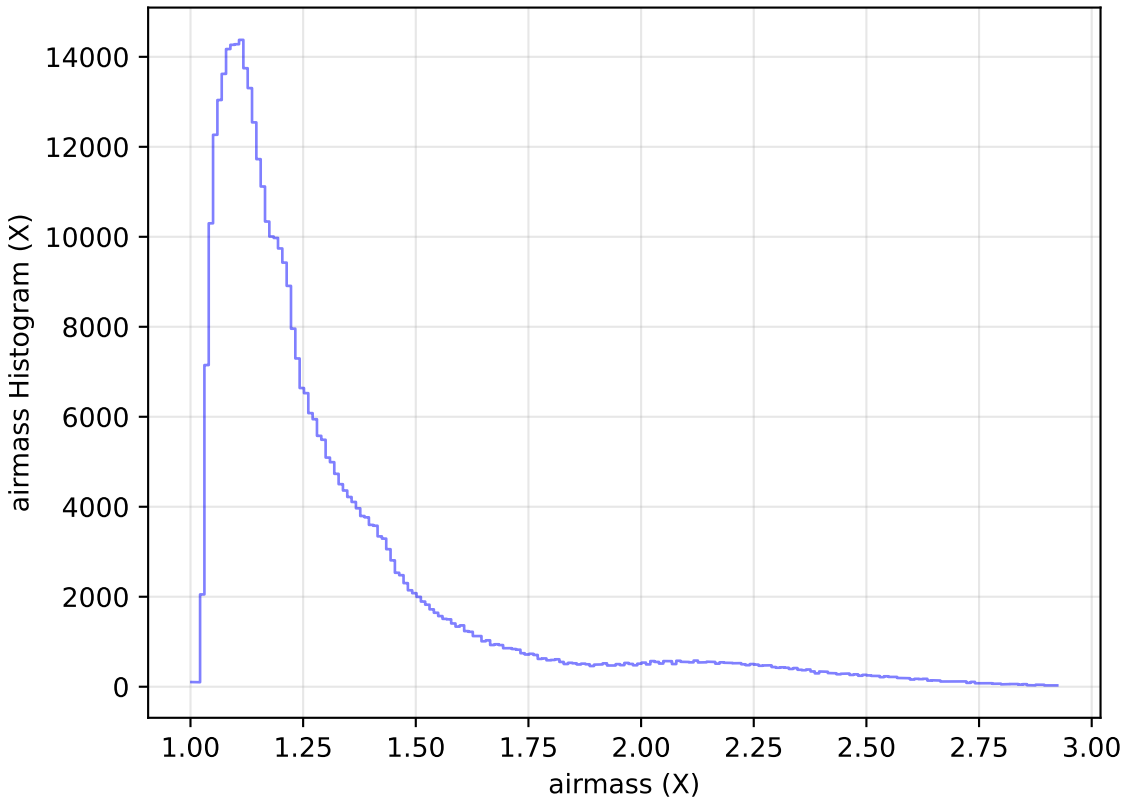
roll_pause_mjdp270_v3.4_10yrs All sky z band: airmass Histogram
