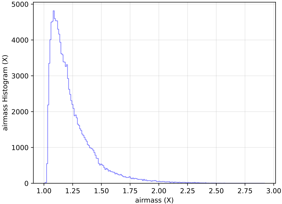
roll_pause_mjdp270_v3.4_10yrs All sky u band: airmass Histogram
