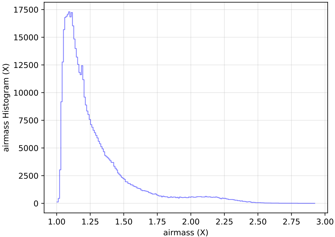
roll_pause_mjdp270_v3.4_10yrs All sky r band: airmass Histogram
