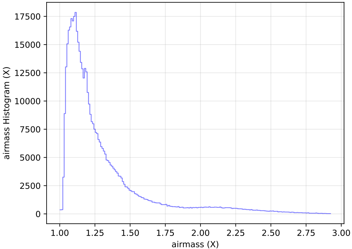
roll_pause_mjdp270_v3.4_10yrs All sky i band: airmass Histogram
