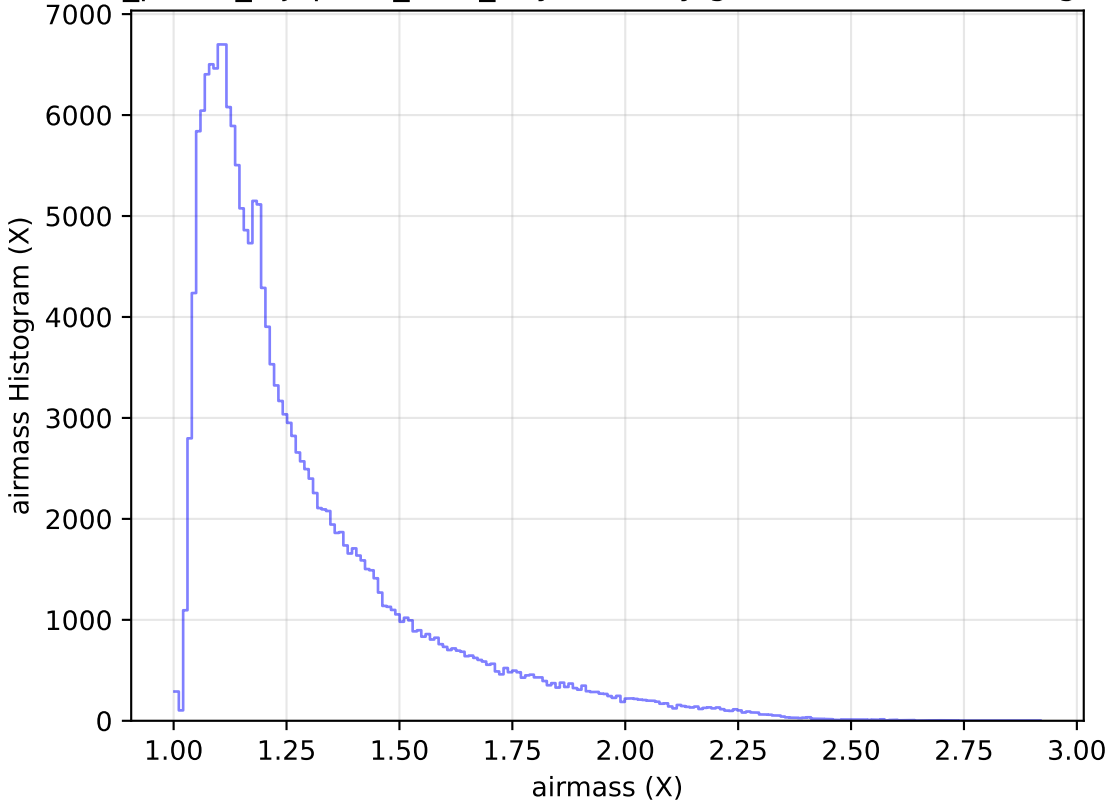
roll_pause_mjdp270_v3.4_10yrs All sky g band: airmass Histogram
