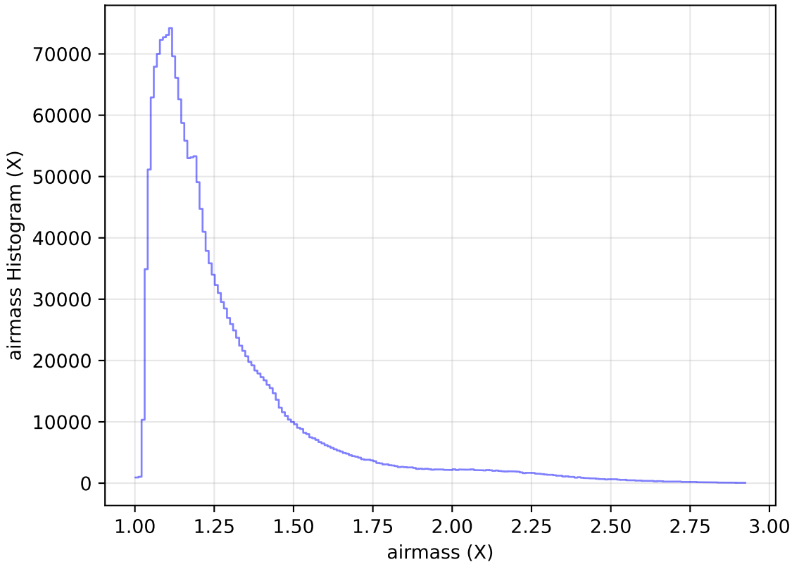
roll_pause_mjdp270_v3.4_10yrs All sky all bands: airmass Histogram
