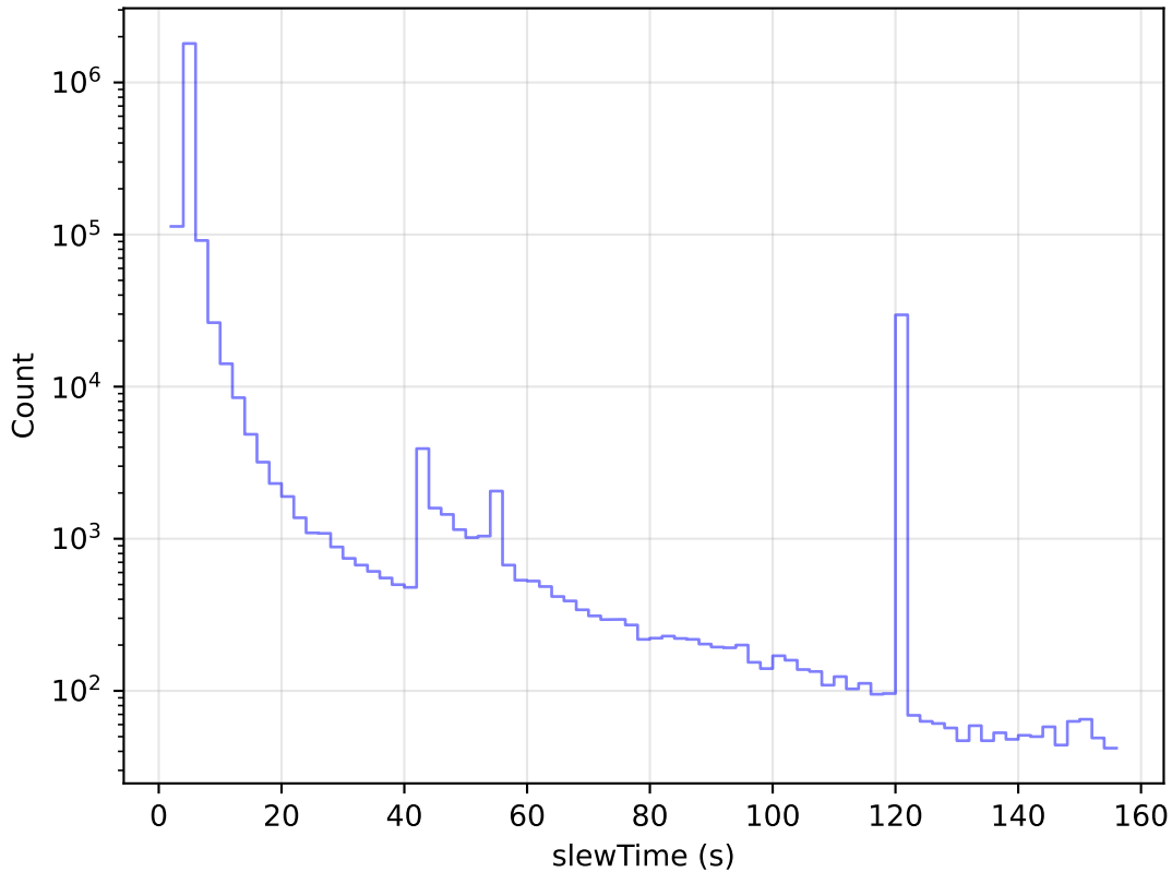
roll_pause_mjdp270_v3.4_10yrs All visits: Slew Time Histogram
