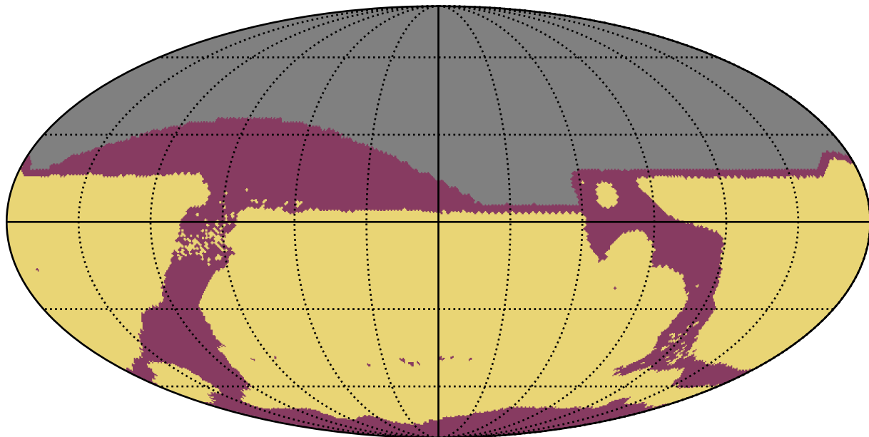
roll_pause_mjdp270_v3.4_10yrs All sky: RapidRevisits
