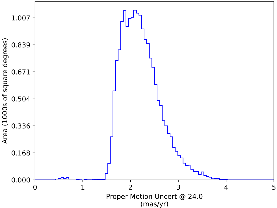
roll_pause_mjdp270_v3.4_10yrs WFD: Proper Motion Uncert @ 24.0
