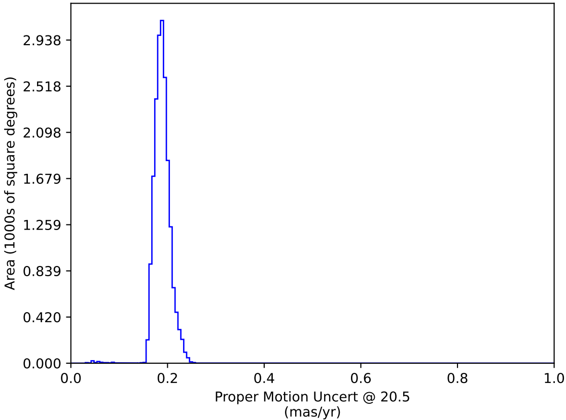
roll_pause_mjdp270_v3.4_10yrs WFD: Proper Motion Uncert @ 20.5
