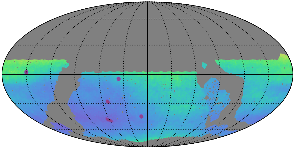
roll_pause_mjdp270_v3.4_10yrs WFD: Parallax Uncert @ 24.0
