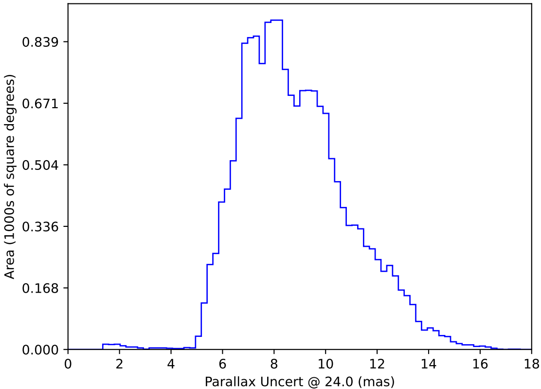
roll_pause_mjdp270_v3.4_10yrs WFD: Parallax Uncert @ 24.0
